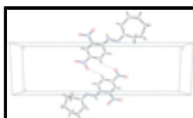
Fig. 2. The crystal packing of the title compound, viewed down the c -axis showing dimer formation. Intermolecular hydrogen bonds are shown as dashed lines.
