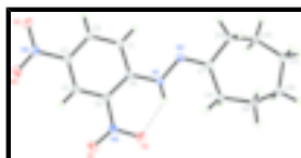
Fig. 1. View of the molecular structure of the title compound with atom labels and 50% probability ellipsoids for non-H atoms. Intramolecular hydrogen bond is shown as dash lines.
